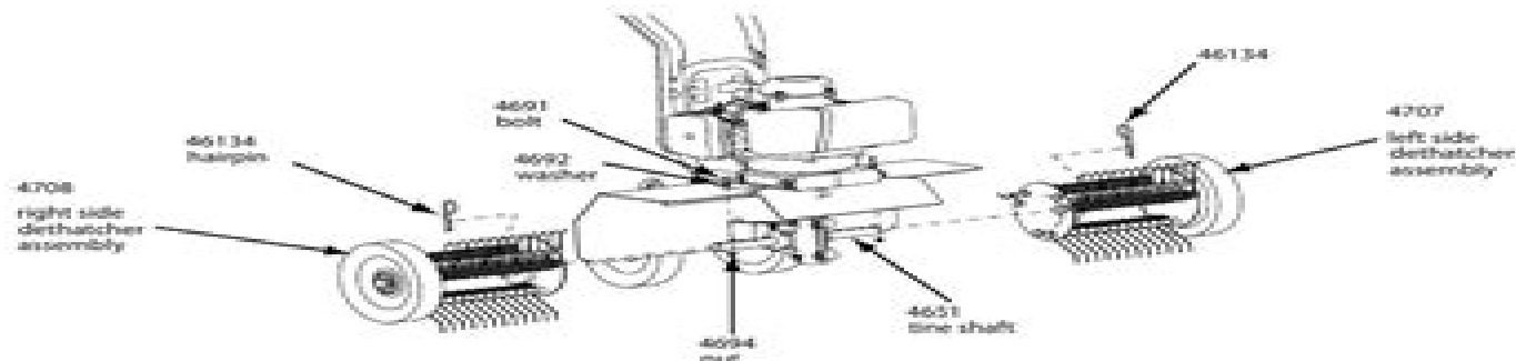
DK43 Dethatcher Kit (fits both Models MC43 & MC43E or stand-alone as MD43)
