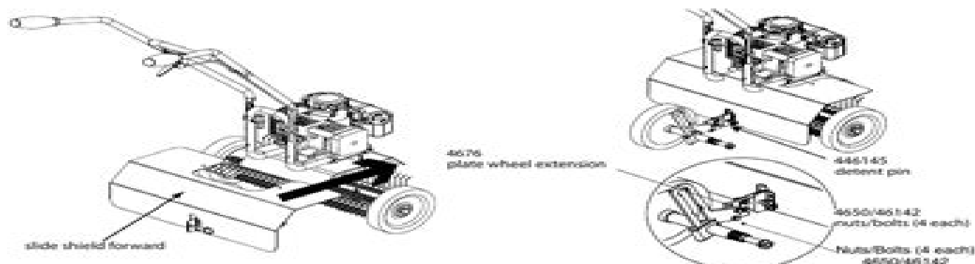
DK43 Dethatcher Kit (fits both Models MC43 & MC43E or stand-alone as MD43)
