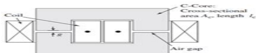
Figure 3.35 C-core inductor for Problem 3.18.
