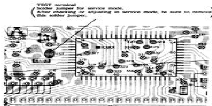
Fig.4 TEST terminal position
