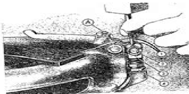
Fig. 84. - Stripping of clutch on device A 711063/A.
