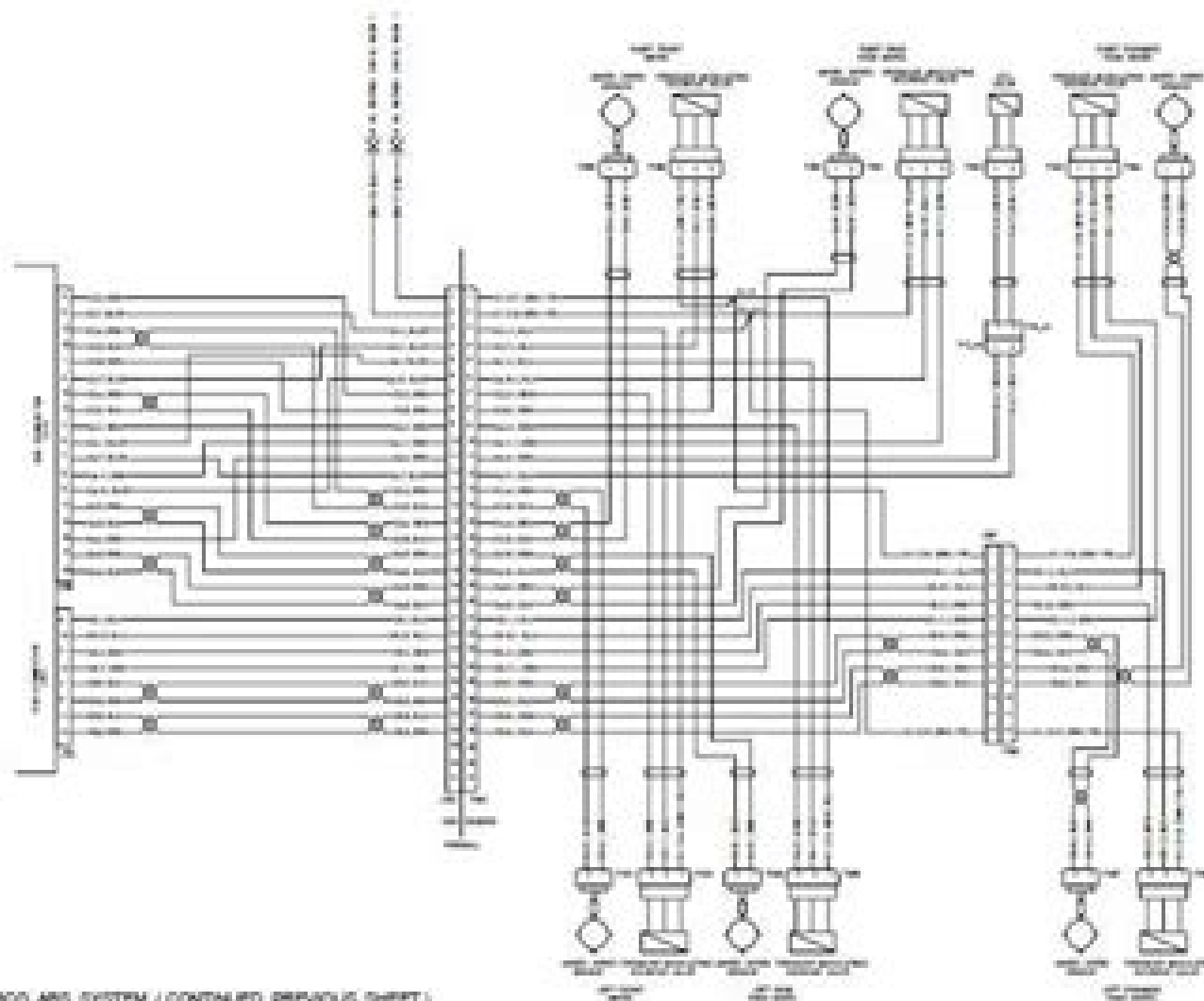
WABCO ABS SYSTEM (CONTAINED PREVIOUS SHEET)
