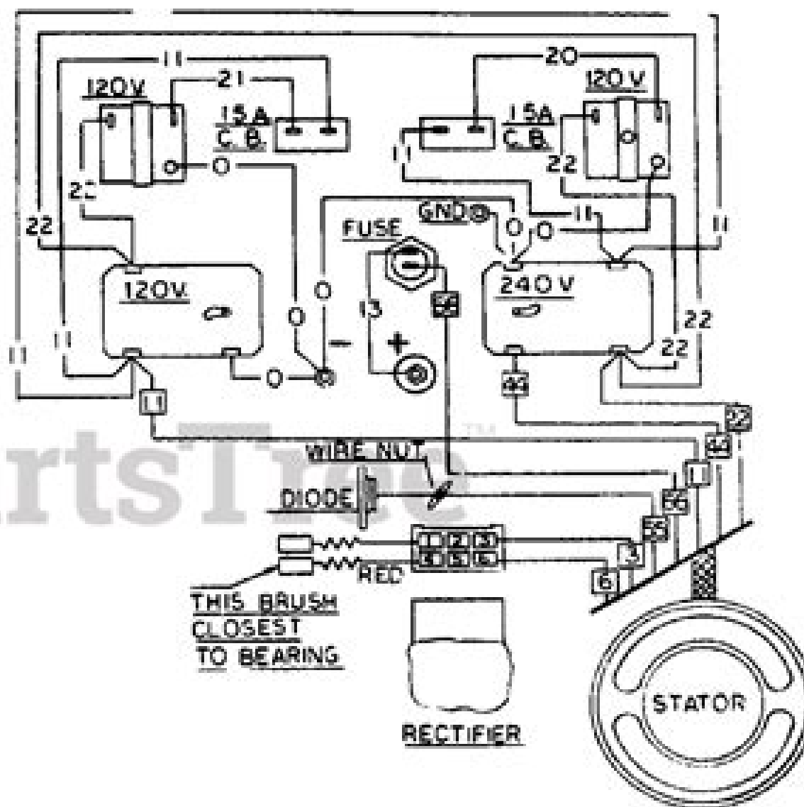
ELECTRICAL SCHEMATIC/WIRING DIAGRAM MANUAL START UNITS
