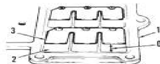
Fig. S211-5—View identifying reed plate (1), reed valves (2) and reed stops (3). Reed stop opening (D) should be 0.0-0.4 mm (0.00-0.02 in.).
