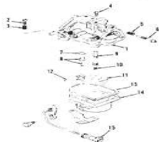
Fig. S211-1—Exploded view of Mikuni B32-28 carburetor.
