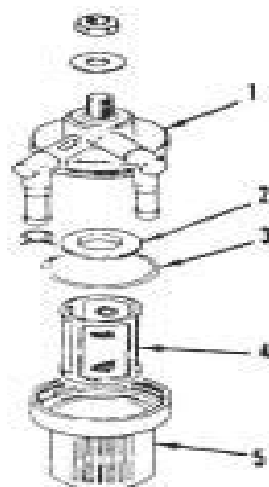
Fig. S211-3—Exploded view of fuel filter assembly.
