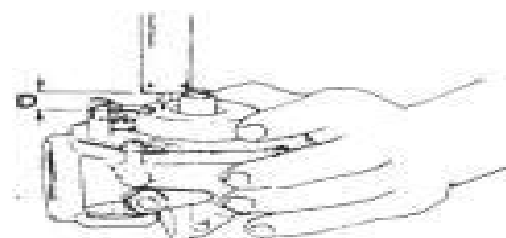
Fig. S211-2—Distance (D) for correct float level should be 10-12 mm (0.394-0.472 in.).
