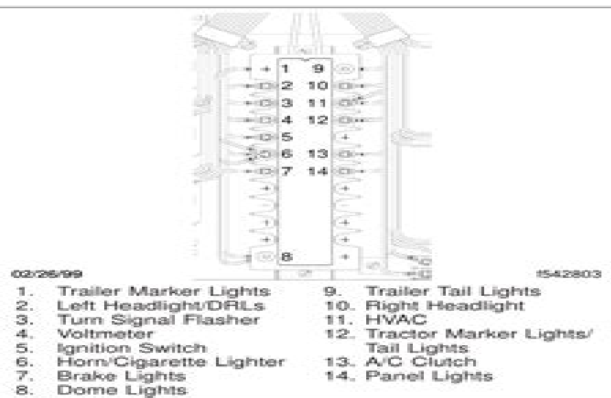
Fig. 3.8, Circuit Breaker Layout (detail)
