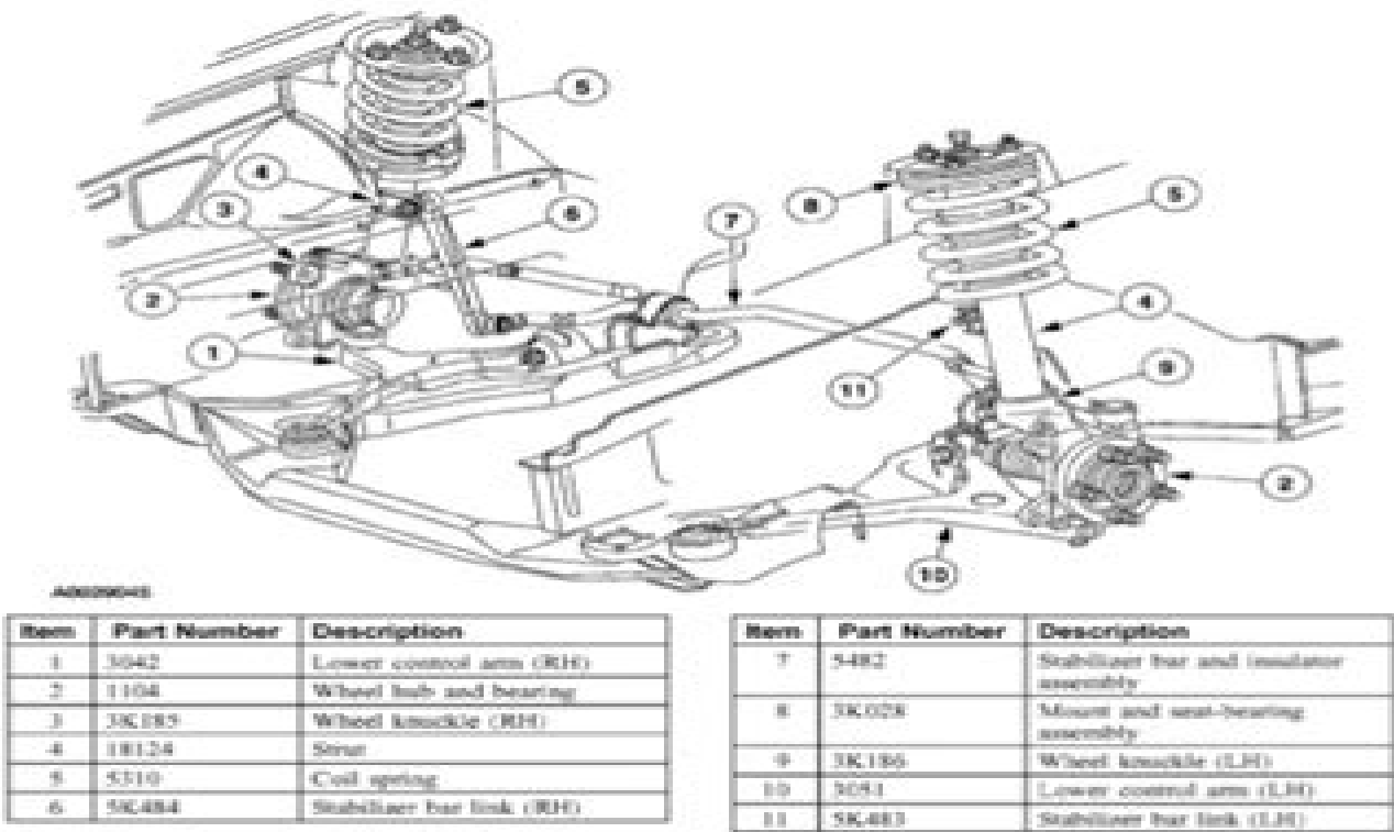
Fig. 1: Identifying Taurus/Sable Front Suspension Components Courtesy of FORD MOTOR CO.
