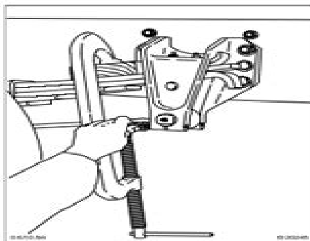
Fig. 3. Remove the Pinch Bolts
