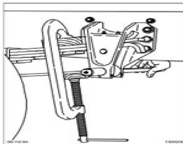
Fig. 4. Tap the Eye Pin Out
