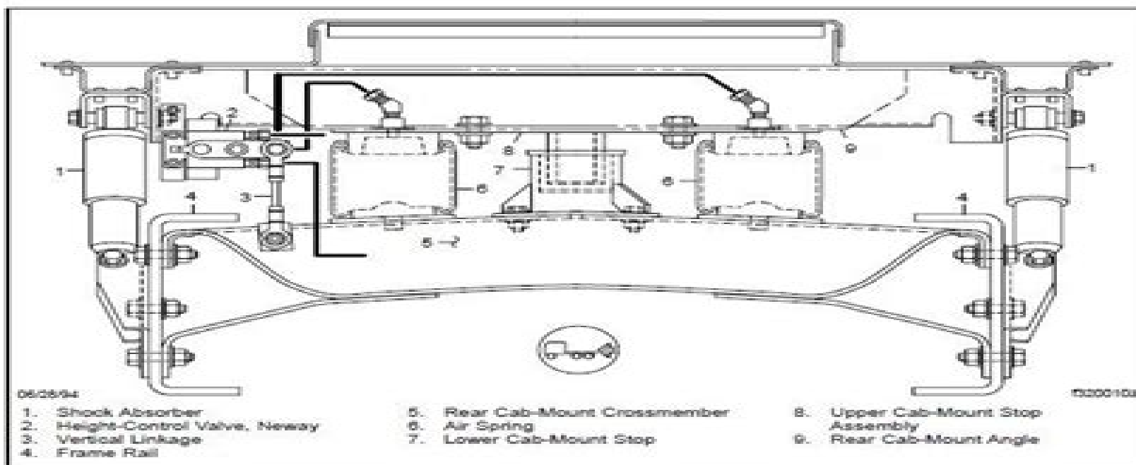
Fig. 4, Cab Rear Air-Suspension Installation, Vehicles Built From January 1990 to April 1991 (without lateral control rod)
