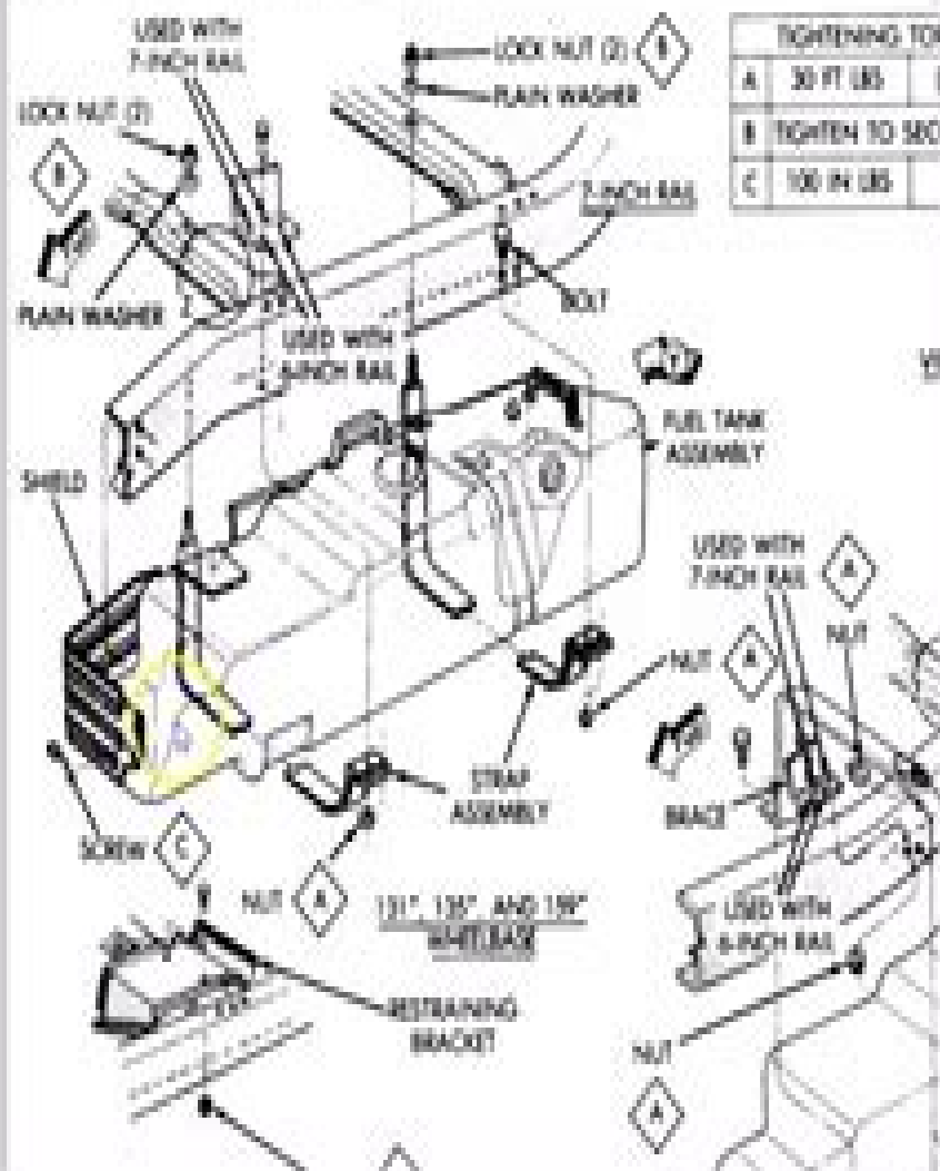
Fig. 1 Common components of the rear lower mounted fuel tank
