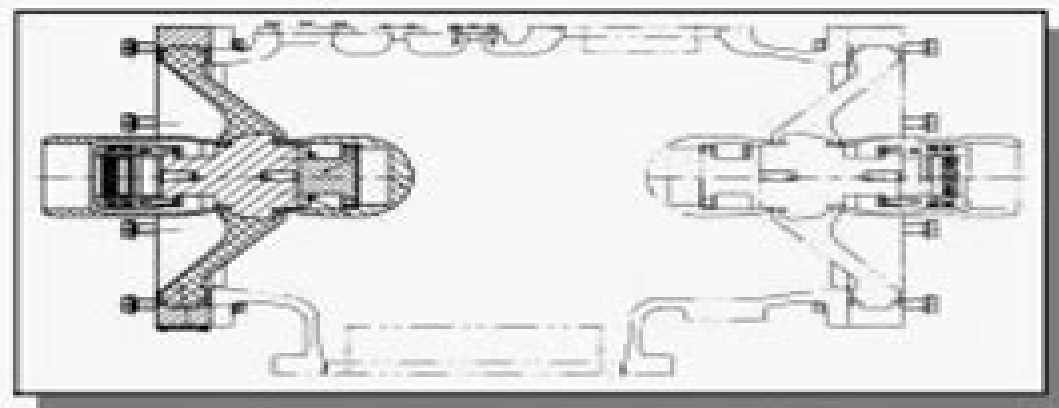
Buffer compartment without Busbar link
