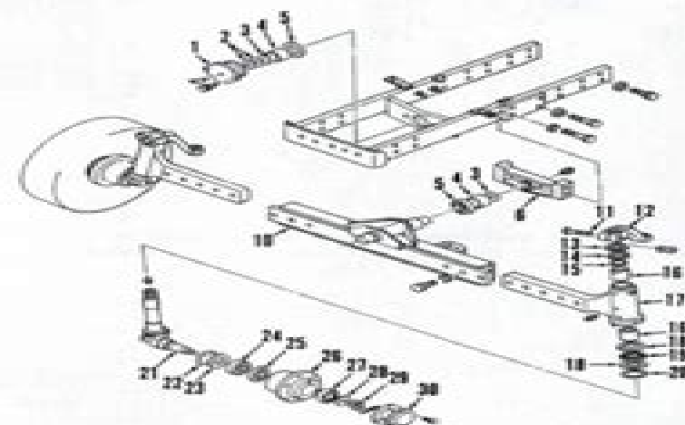
Fig. 4—Exploded view of adjustable tread width front axle assembly used on Model 1520. Refer to Fig. 3 for legend except for axle extension (17).
