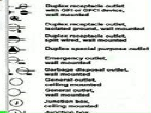
Outlet symbols
