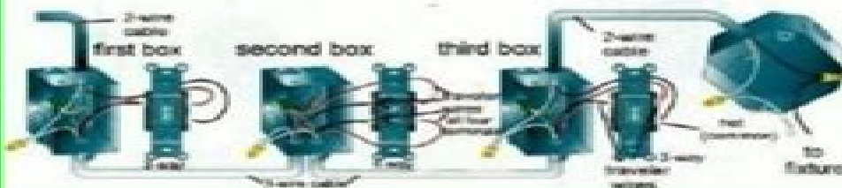
4-way switch
