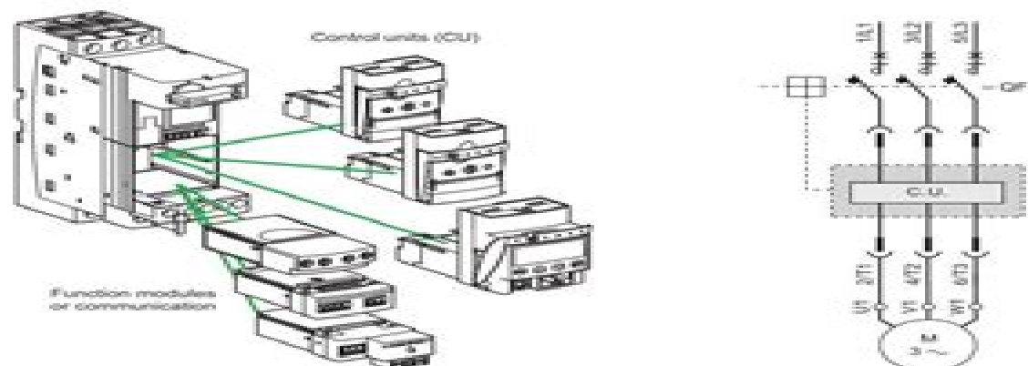
Fig. N71 : Example of a GPS modularity (TeSys U starter controller by Schneider Electric)
